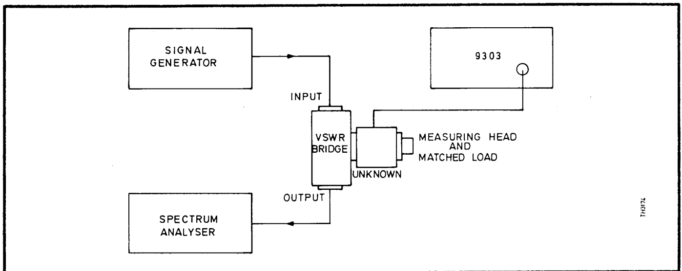
Fig. 6.3 Connections for VSWR Check
