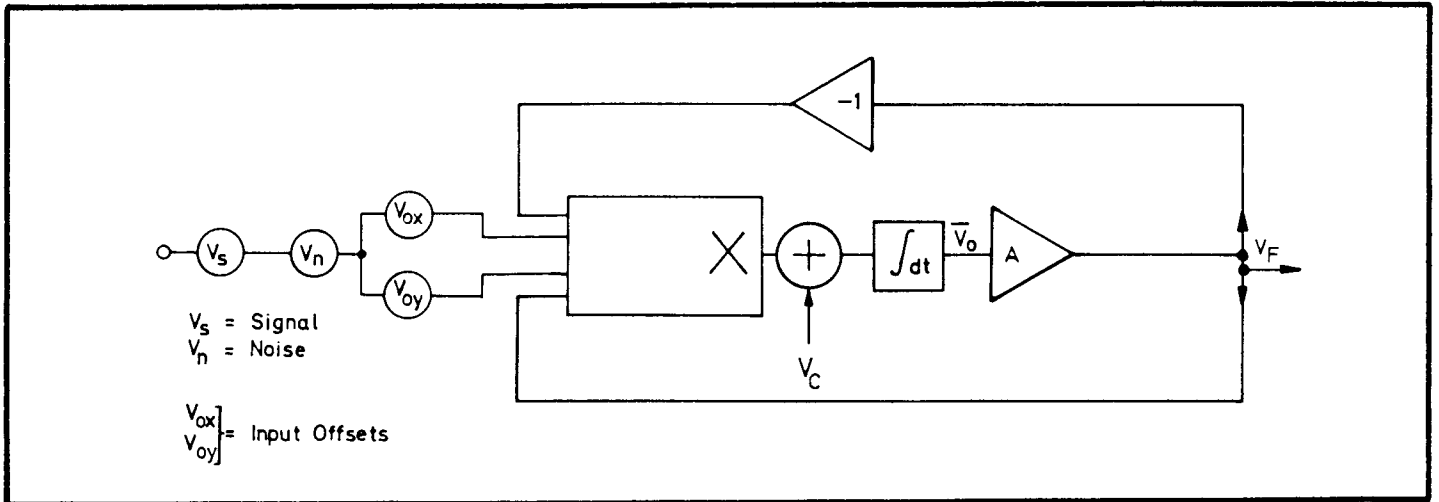
Fig. 5.7 Feedback Loop
