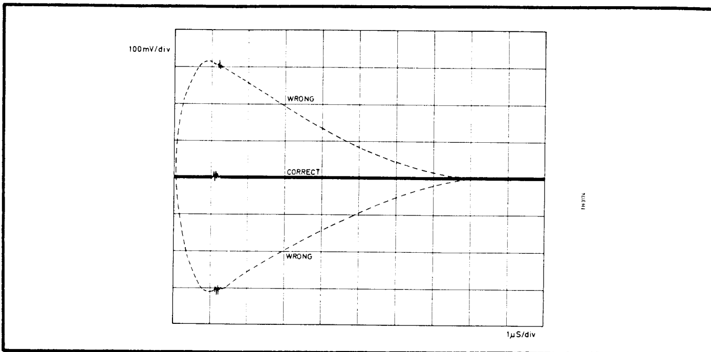
Fig. 6.2 Bias Balance Waveform
