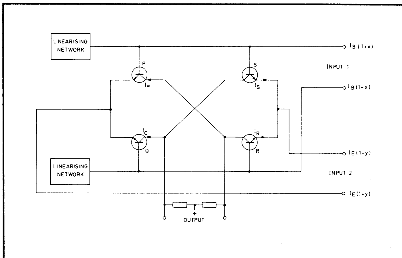
Fig. 5.8 Multiplier Operation
