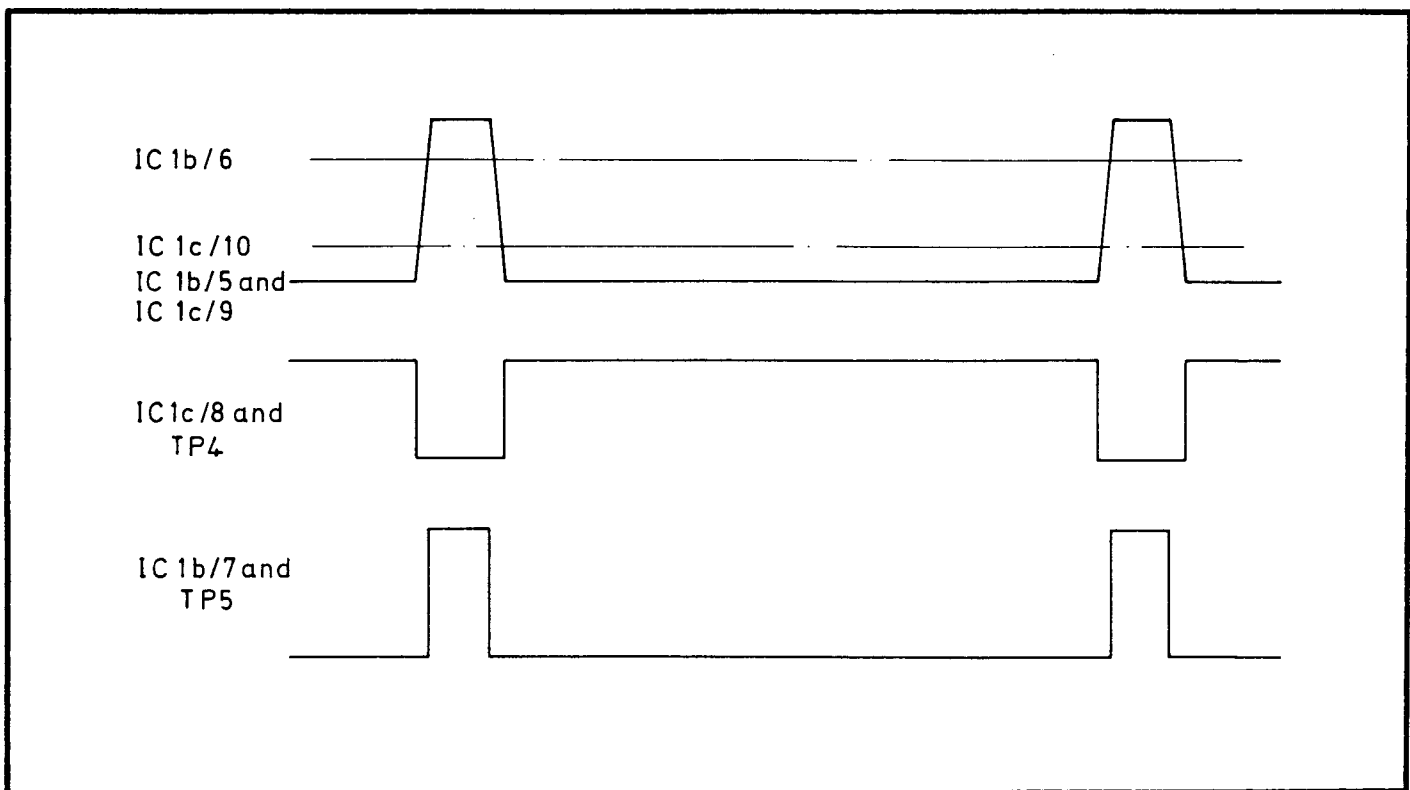
Fig. 5.6 Comparator Waveforms
