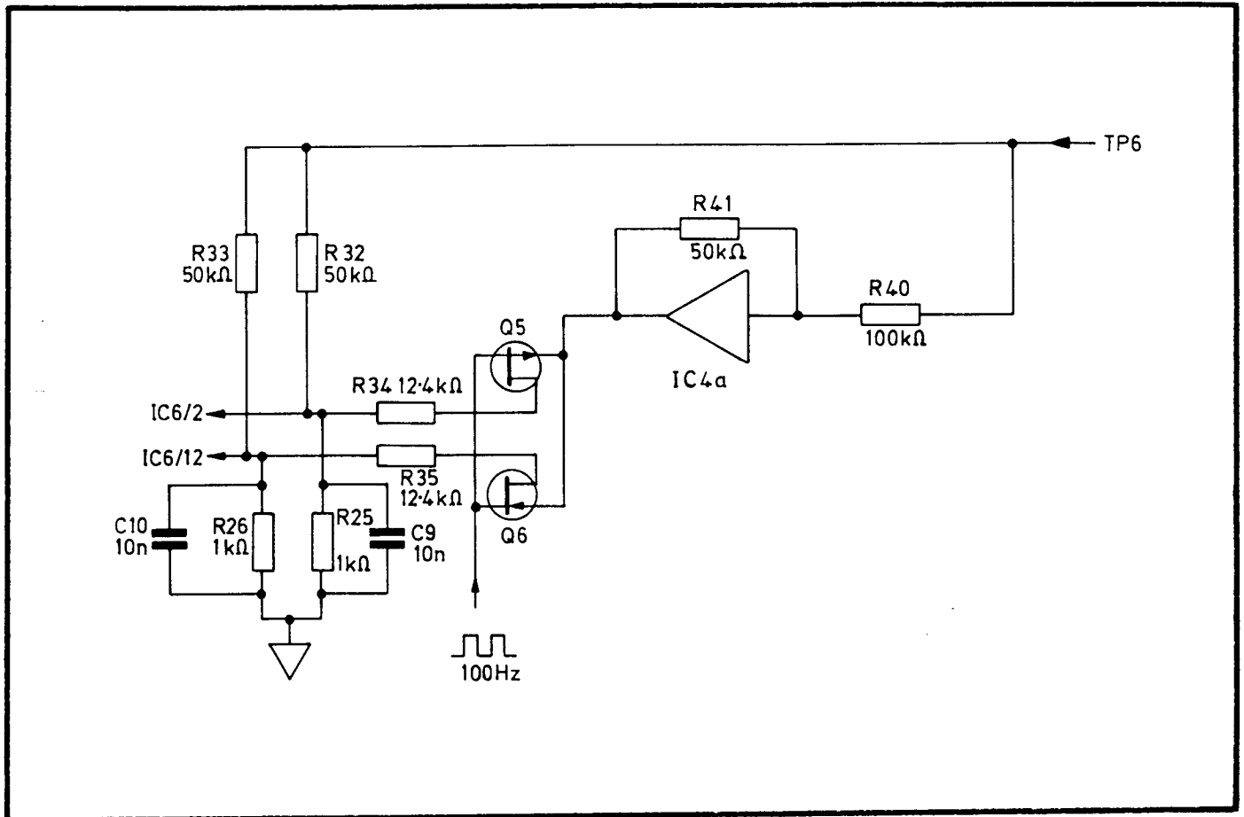
Fig. 5.5 Feedback Switching
