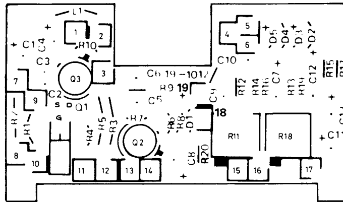
ASSEMBLY 19-1012
