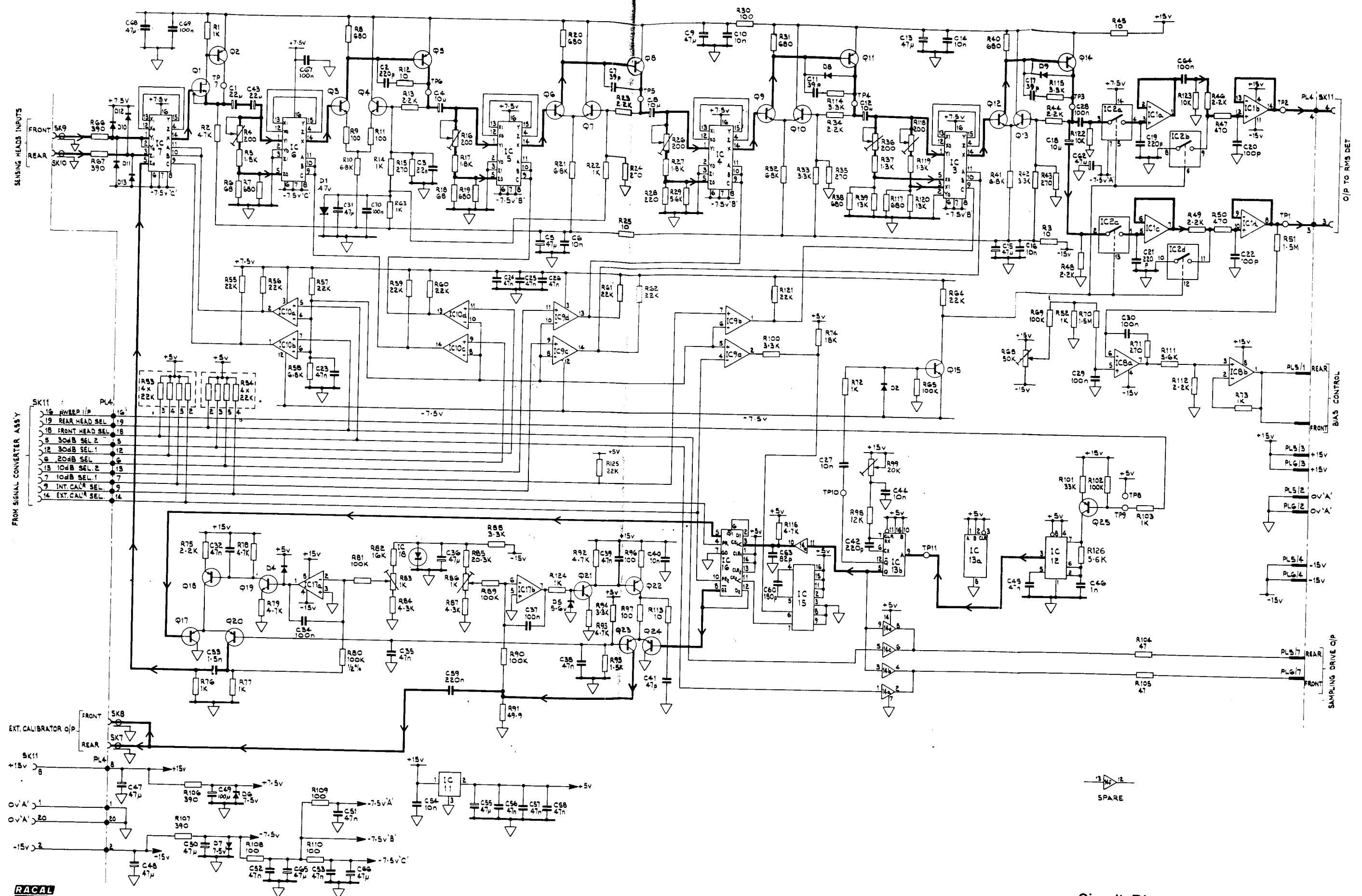
Circuit Diagram: Fig.11 Amplifier Assembly 19-1016
